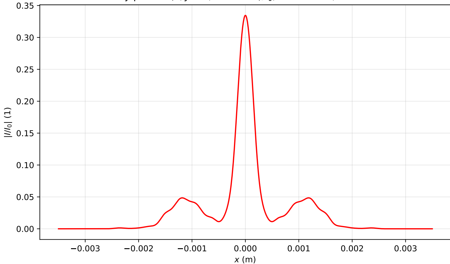
Intensity profile I(x, y = 0, z = 2.866)/I_0 , \text{Pin}=8.5\text{Pcr} , artificial time
